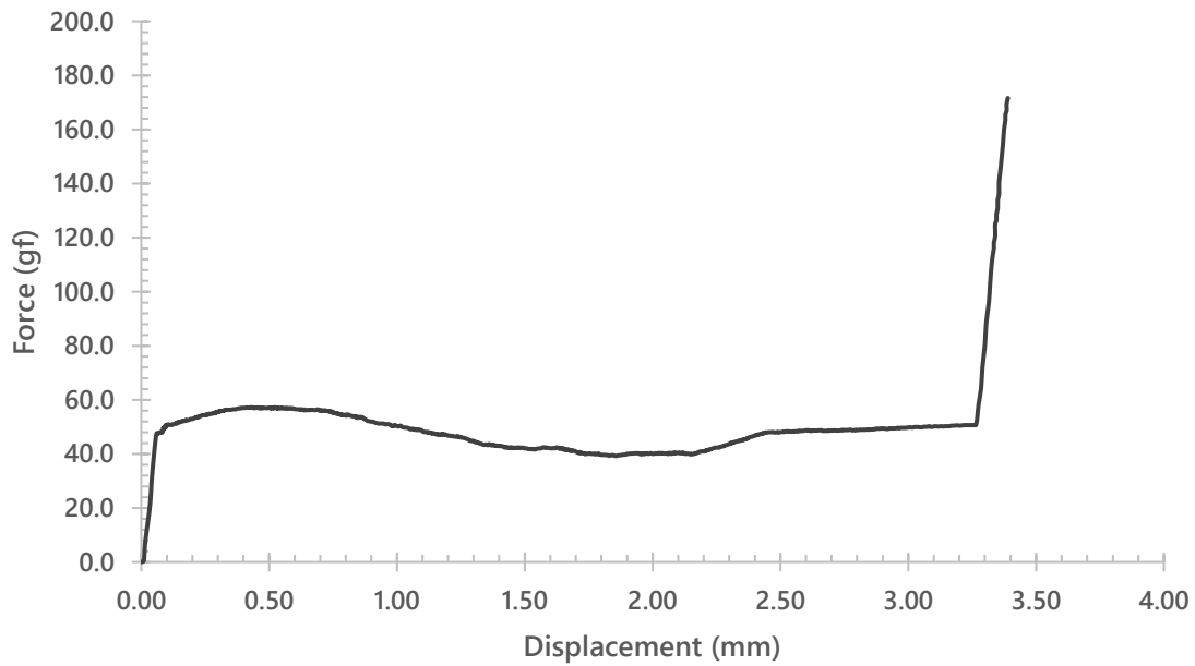
Gateron Banana Jelly (Upstroke)
